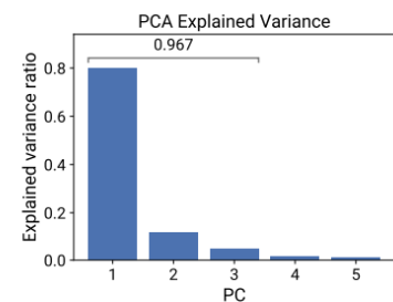
(a) PCA explained variance
